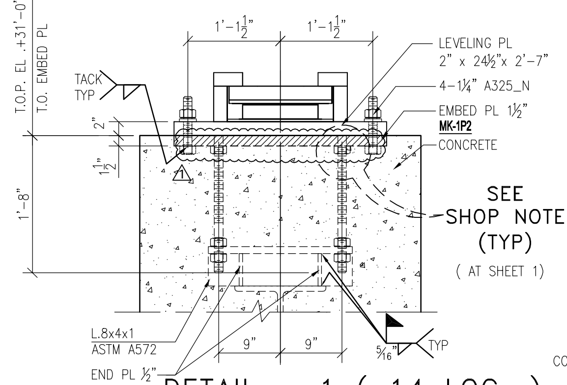
DETAIL - 1 ( 14 LOC. )
